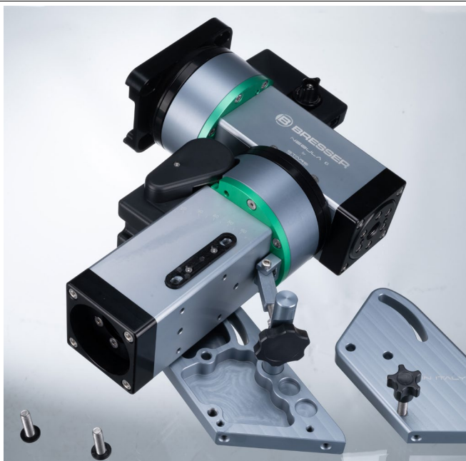
Remove one of the two lateral bracket
